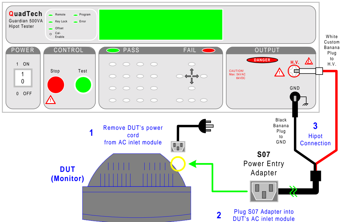
Figure 1: Guardian 500VA Hipot Tester
